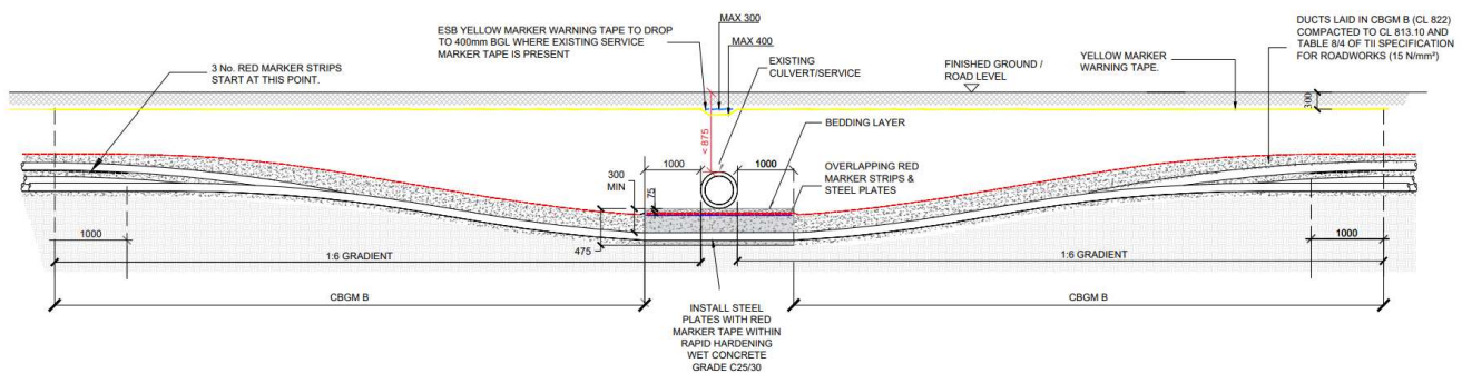
Figure 9 - 38kV UGC Culvert Undercrossing
